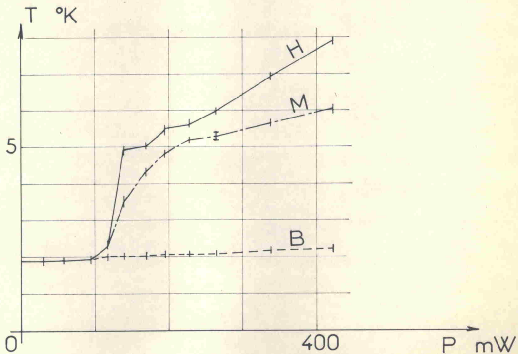
FIG.8 : Superfluid helium T = 1.85 K ; p = 3.5 atm
